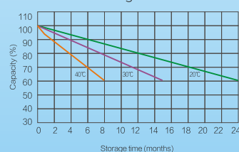
Self-discharge characteristic
