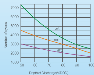
Cycle life vevurs DOD and tempture at 0.2C
