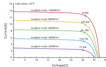
Current-Voltage Curve
