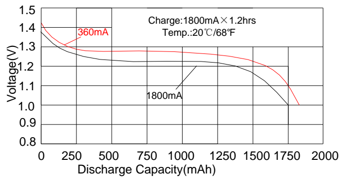
Discharge characteristics
