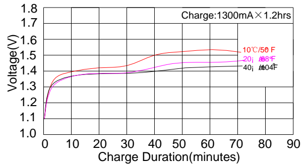
Fast charge characteristics
