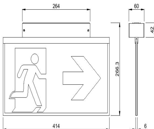
Dimensional sketch (mm)
