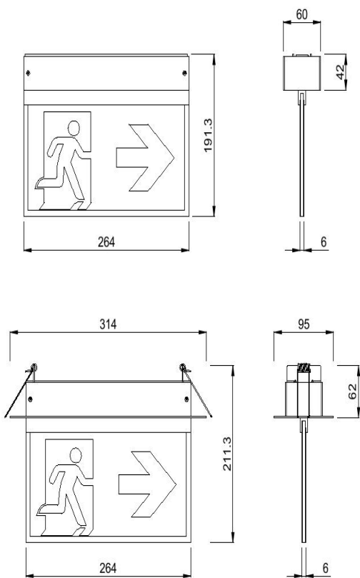
Dimensional sketch (mm)
